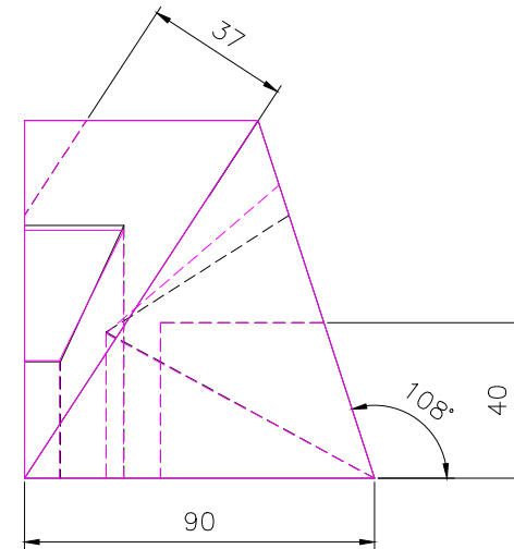
RIGHT SCALE 1/2
