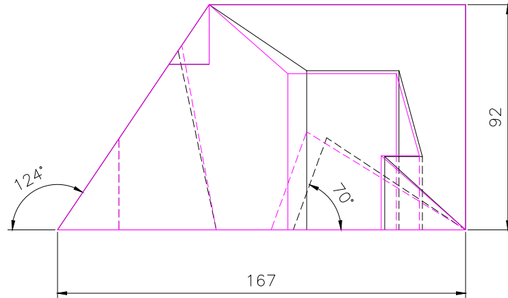
FRONT SCALE 1/2
