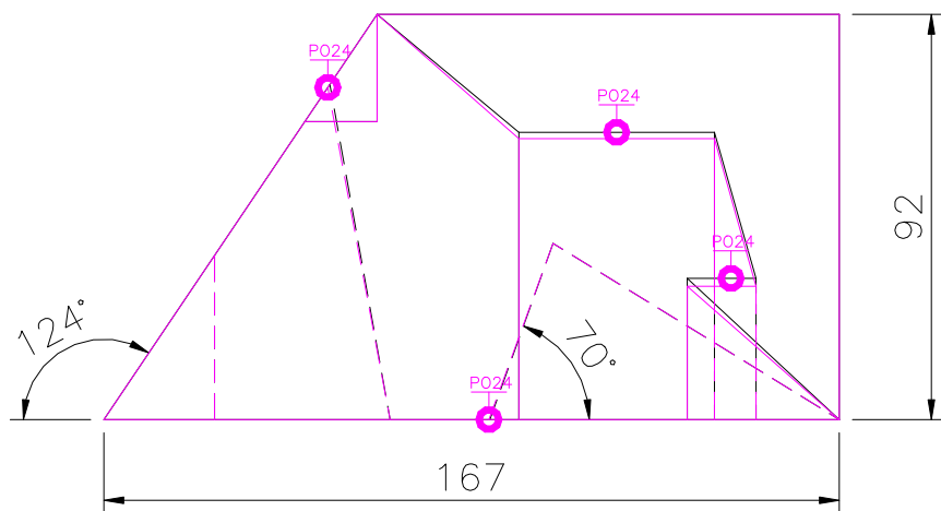
FRONT SCALE 1/2
