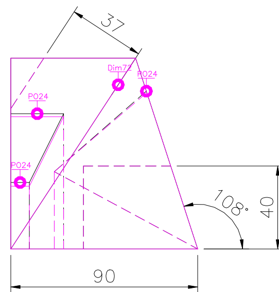
RIGHT SCALE 1/2
