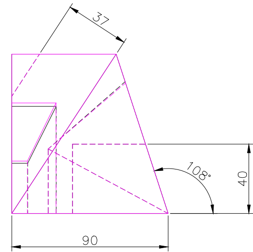
RIGHT SCALE 1/2
