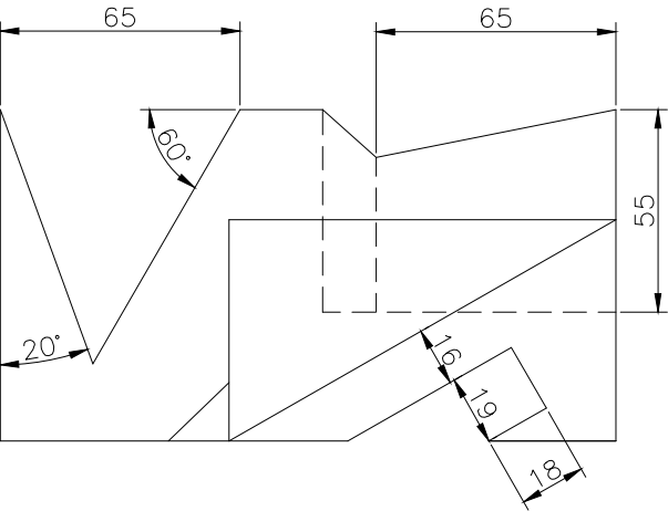
TOP SCALE 1/2
