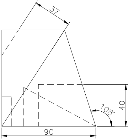
RIGHT SCALE 1/2
