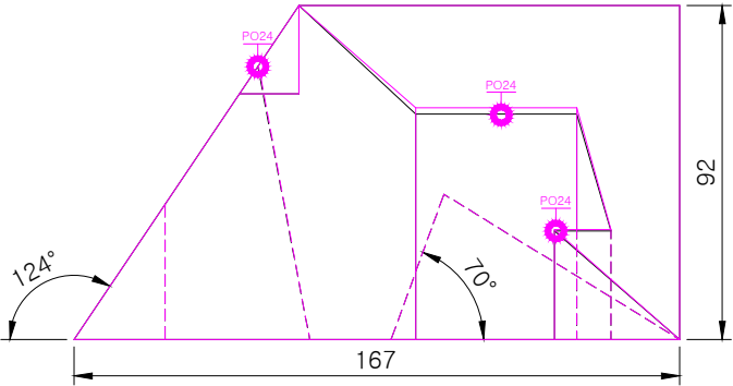
FRONT SCALE 1/2
