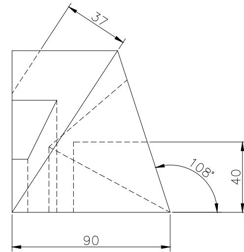
RIGHT SCALE 1/2
