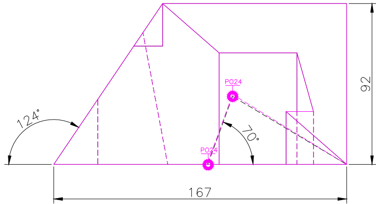
FRONT SCALE 1/2
