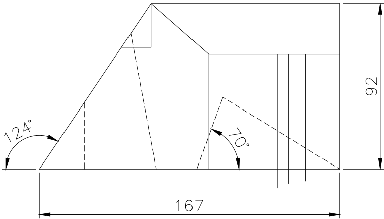
TOP SCALE 1/2
