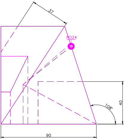
RIGHT SCALE 1/2
