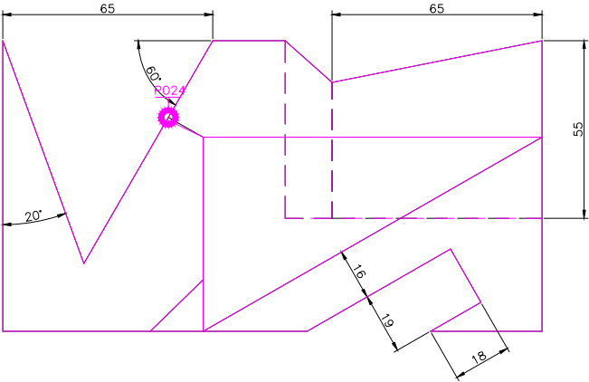
TOP SCALE 1/2
