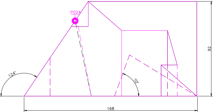
FRONT SCALE 1/2
