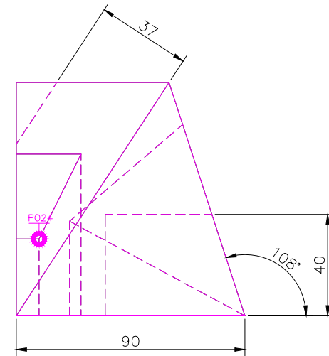
RIGHT SCALE 1/2
