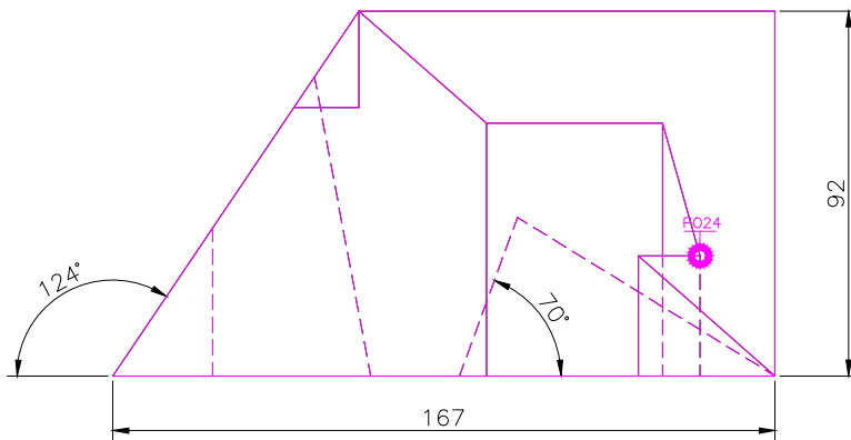
FRONT SCALE 1/2
