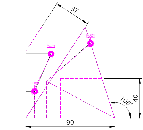
RIGHT SCALE 1/2
