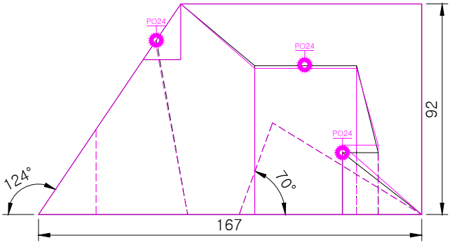
FRONT SCALE 1/2
