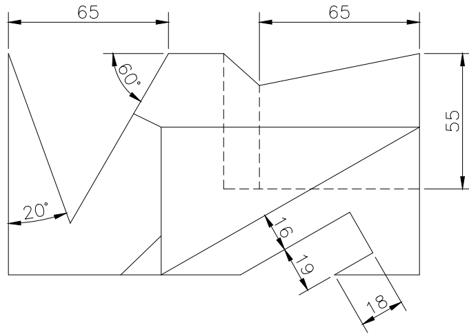
TOP SCALE 1/2
