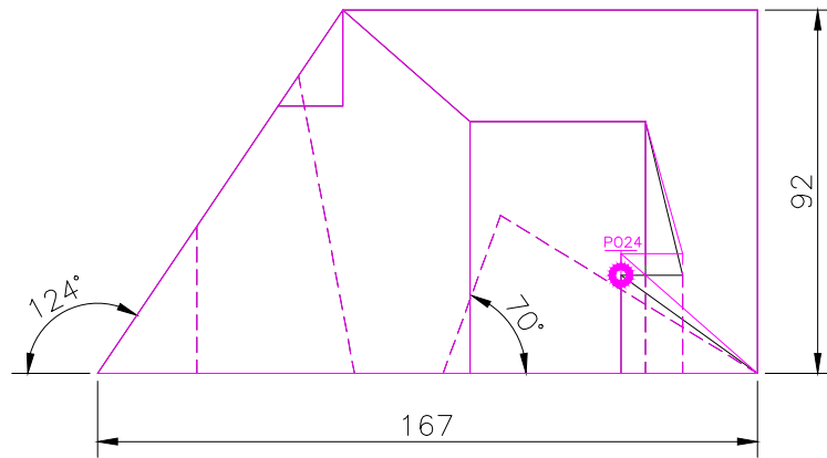
FRONT SCALE 1/2
