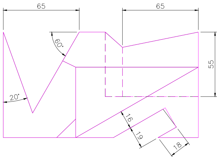
TOP SCALE 1/2
