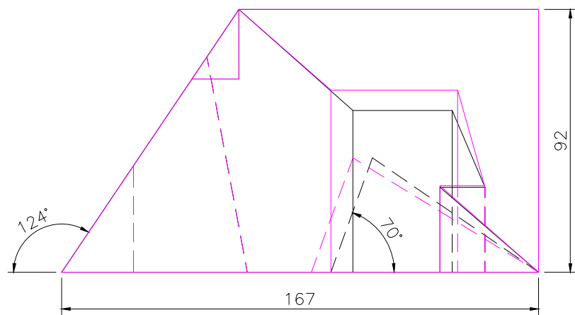
FRONT SCALE 1/2
