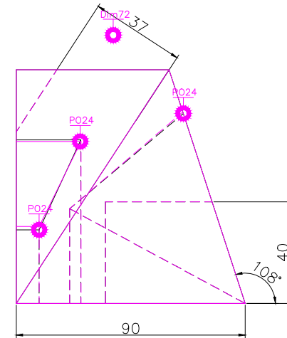
RIGHT SCALE 1/2
