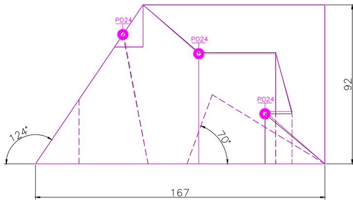
FRONT SCALE 1/2
