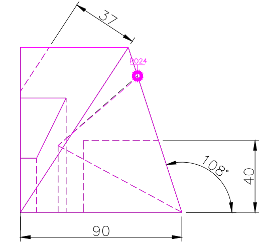
RIGHT SCALE 1/2
