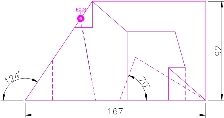
FRONT SCALE 1/2
