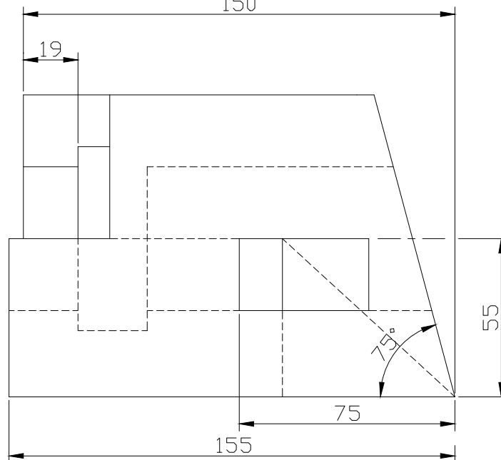
FRONT SCALE 1/2
