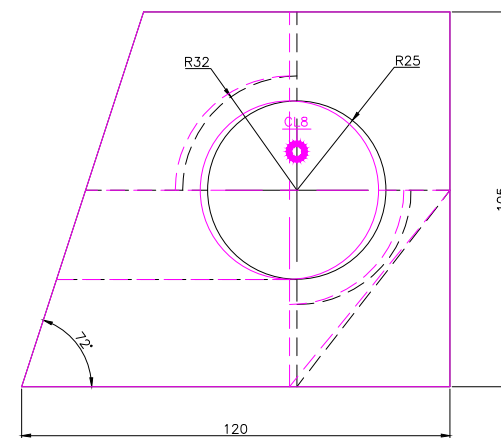
RIGHT SCALE 1/2
