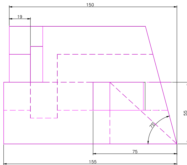
FRONT SCALE 1/2
