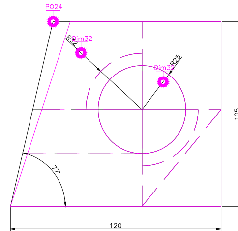
RIGHT SCALE 1/2
