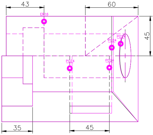
TOP SCALE 1/2
