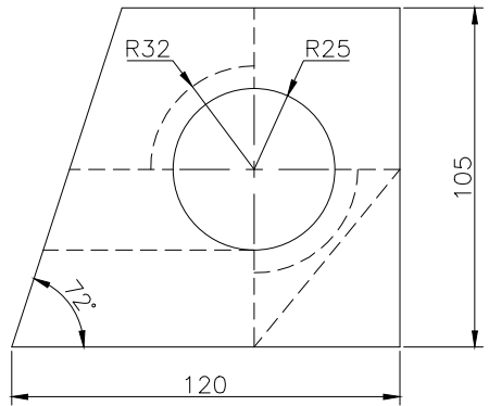
RIGHT SCALE 1/2
