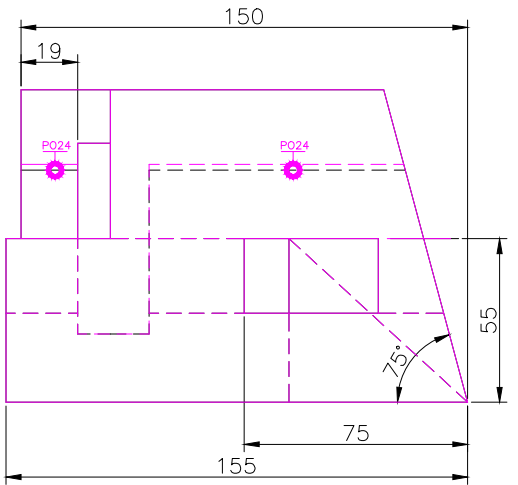
FRONT SCALE 1/2
