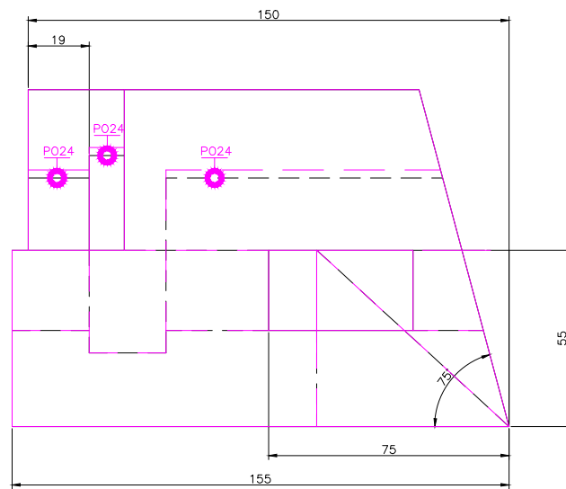
FRONT SCALE 1/2
