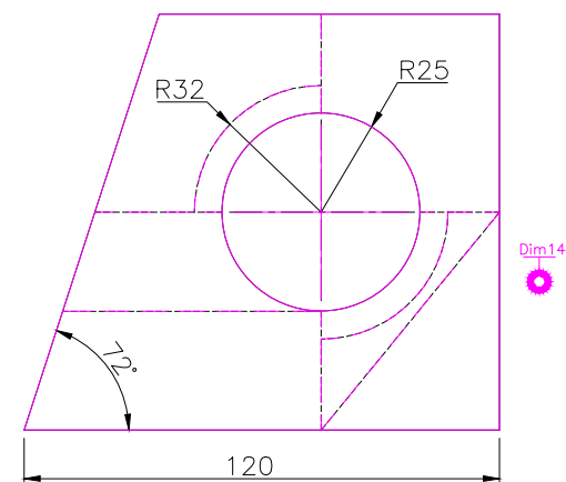
Right SCALE 1/2
