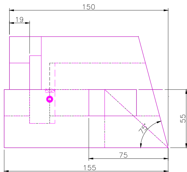
Front SCALE 1/2
