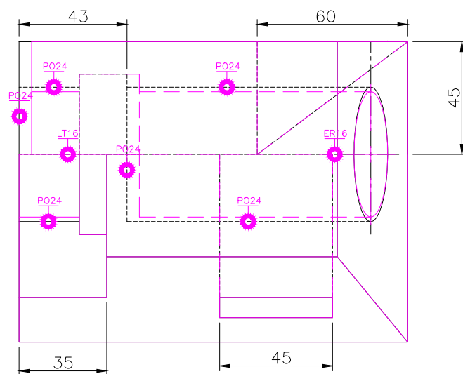
Top SCALE 1/2
