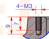
"상세뷰 C (1:1)"
