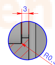
"상세뷰 D (1:1)"
