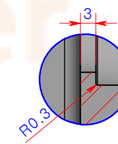
"상세뷰 E (1:1)"
