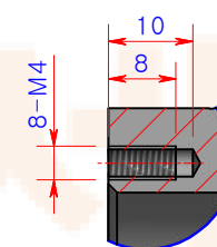
"상세뷰 B (1:1)"
