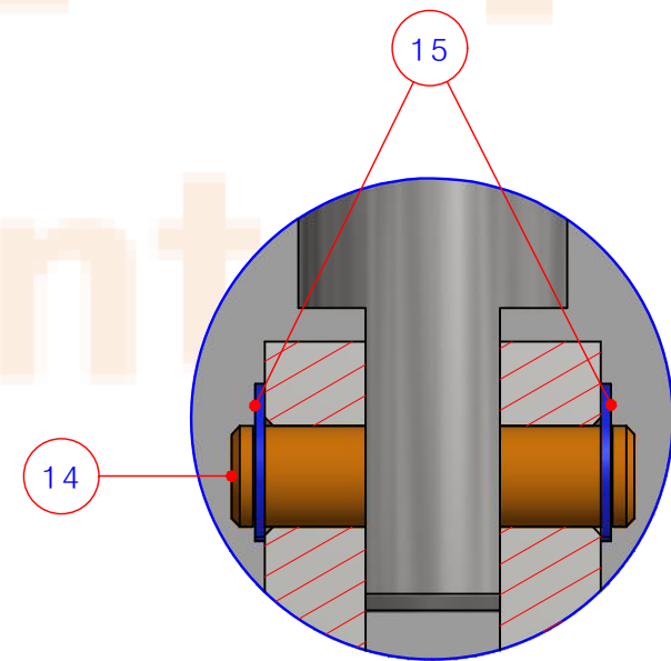
"상세뷰 B (2:1)"
