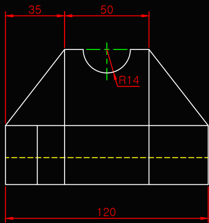
RIGHT
