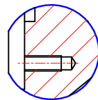
"상세뷰C ( 1 : 1 )"
